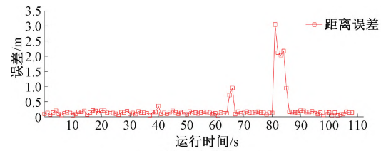
(a) 本文方法 (a) The proposed method
