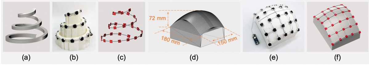
Fig. 6. (a) The 3D model of a conical spiral. (b) The 3D printed model of a conical spiral attached with the sensor network. (c) The virtual model reconstructed by the sensor network. (d) The 3D model of a rotational paraboloid. (e) The 3D printed model of a rotational paraboloid attached with the sensor network. (f) The virtual model reconstructed by the sensor network.
