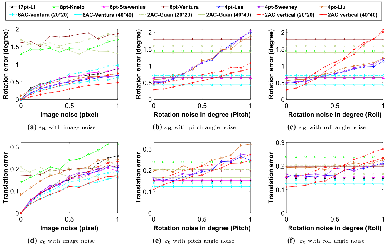
Fig. 11 Rotation and translation error under sideways motion with known vertical direction. Upper row: rotation error. Bottom row: translation error. a, d varying image noise. b, e and c, f varying IMU angle noise and fixed 0.5 pixel std. image noise
