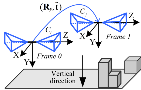
Fig. 4 Relative pose estimation with known vertical direction. There are four unknowns: a y -axis rotation \mathbf{R}_y and 3D translation \mathbf{t} = [\tilde{t}_x, \tilde{t}_y, \tilde{t}_z]^T
