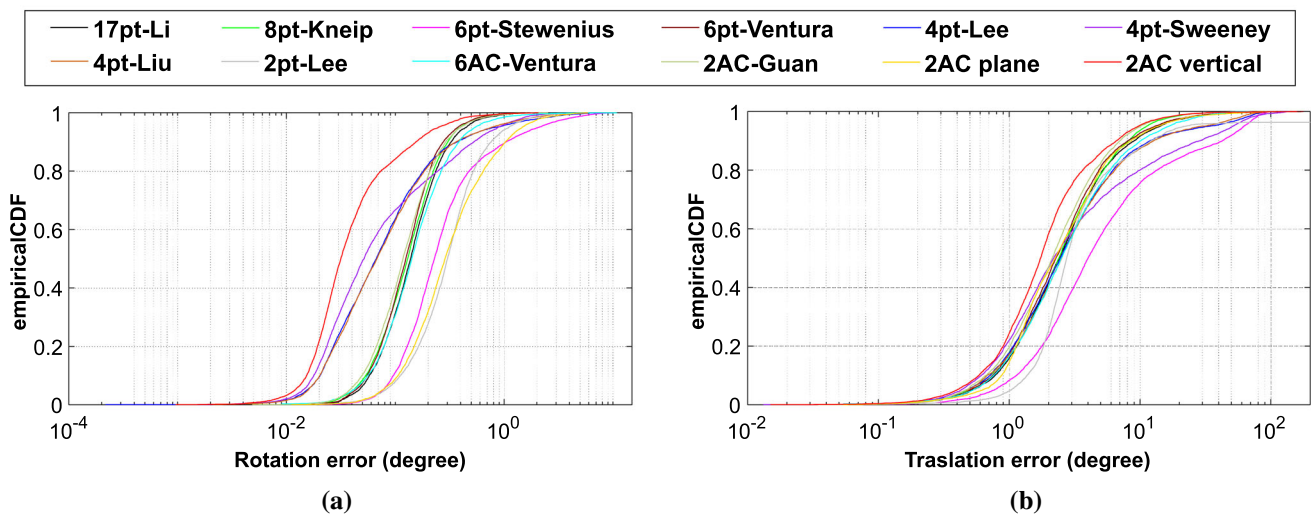
Fig. 15 Empirical cumulative error distributions for KITTI sequence 00. a Reports the rotation error. b Reports the translation error. The proposed 2AC plane method and 2AC vertical are compared against 17pt-Li (Li et al., 2008), 8pt-Kneip (Kneip & Li, 2014), 6pt-Stewenius (Stewenius et al., 2005), 6pt-Ventura (Ventura
