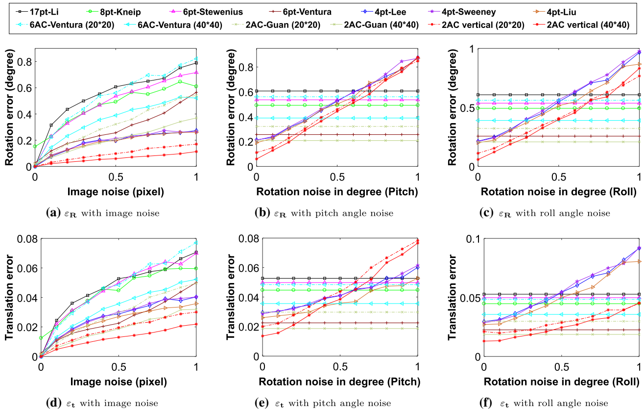
Fig. 13 Rotation and translation error under small rotation motion. Upper row: rotation error. Bottom row: translation error. a, d Varying image noise. b, e and c, f varying IMU angle noise and fixed 0.5 pixel std. image noise
