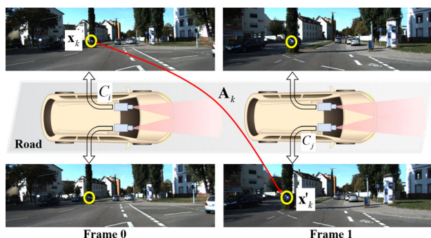
Fig. 1 An affine correspondence in a multi-camera system. It relates two perspective cameras C_i and C_j across two consecutive frames, where C_i and C_j can be the same or different cameras. The local affine transformation A_k relates the infinitesimal patches around correspondence ( x_k, x'_k )
