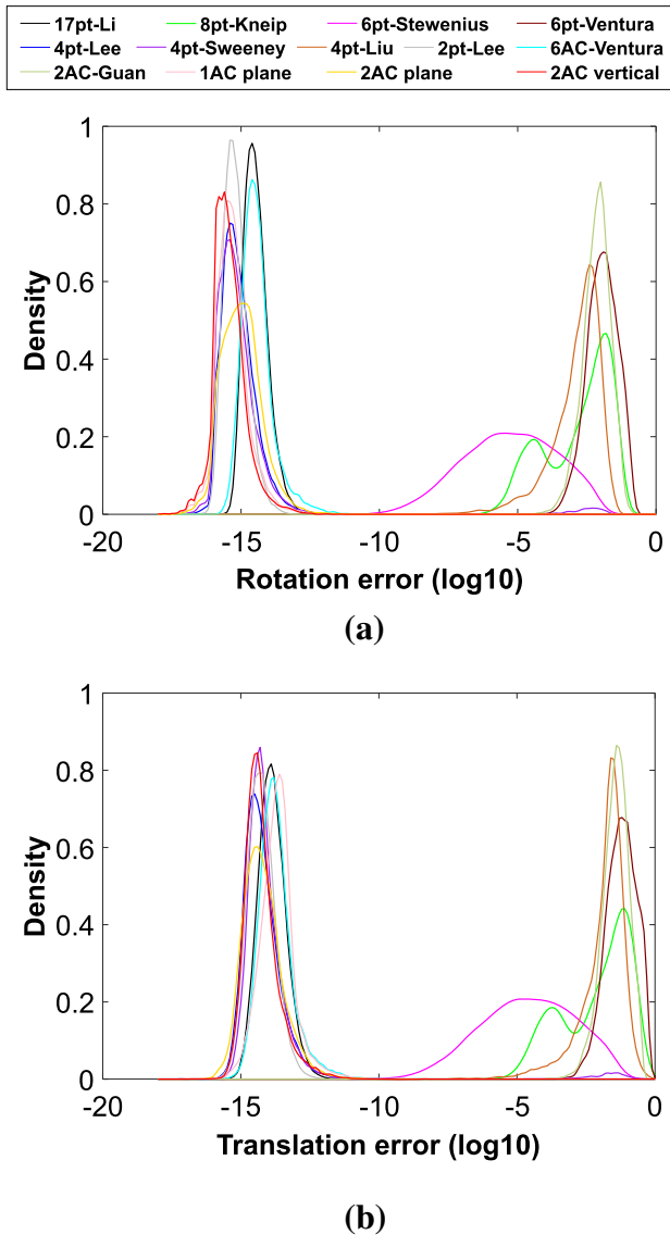
Fig. 5 Probability density functions over estimation errors in the noise-free case (10 000 runs). The horizontal axis represents the \log_{10} errors and the vertical axis represents the density. Plot a reports the rotation error. Plot b reports the translation error. The proposed 1AC plane method, 2AC plane method and 2AC vertical are compared against 17pt-Li (Li et al., 2008), 8pt-Kneip (Kneip & Li, 2014), 6pt-Stewenius (Stewenius et al., 2005), 6pt-Ventura (Ventura et al., 2015), 4pt-Lee (Lee et al., 2014), 4pt-Sweeney (Sweeney et al., 2014), 4pt-Liu (Liu et al., 2017), 2pt-Lee (Lee et al., 2013), 6AC-Ventura (Alyousefi & Ventura, 2020) and 2AC-Guan (Guan et al., 2021a)
