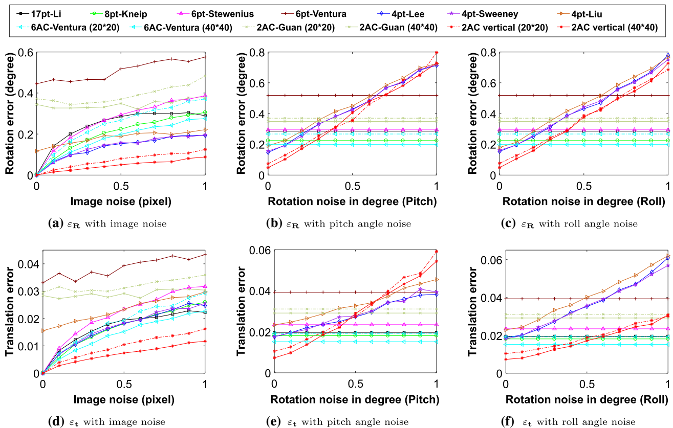
Fig. 10 Rotation and translation error under forward motion with known vertical direction. Upper row: rotation error. Bottom row: translation error. a, d varying image noise. b, e and c, f varying IMU angle noise and fixed 0.5 pixel std. image noise
