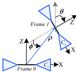
Fig. 2 Relative pose estimation under planar motion in top-view. There are three unknowns: yaw angle \theta , translation direction \phi and translation distance \rho
