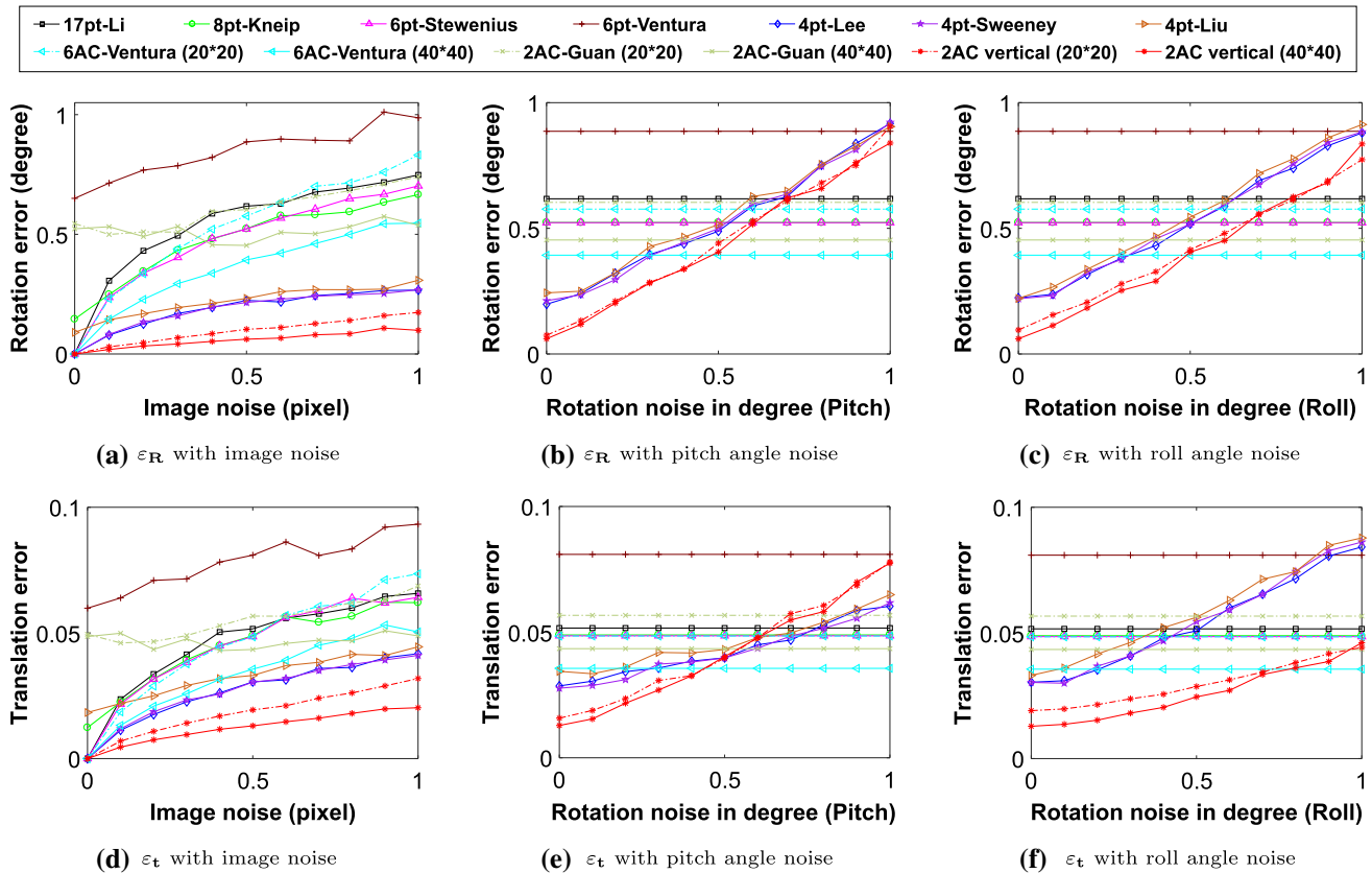
Fig. 9 Rotation and translation error under random motion with known vertical direction. Upper row: rotation error. Bottom row: translation error. a, d varying image noise. b, e and c, f varying IMU angle noise and fixed 0.5 pixel std. image noise
