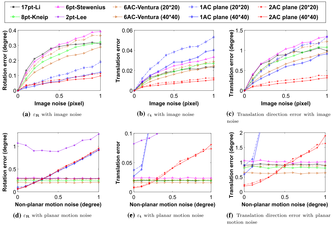
Fig. 6 Rotation and translation error under planar motion. a–c varying image noise under perfect planar motion. d–f varying planar motion noise and fixed 0.5 pixel std. image noise
