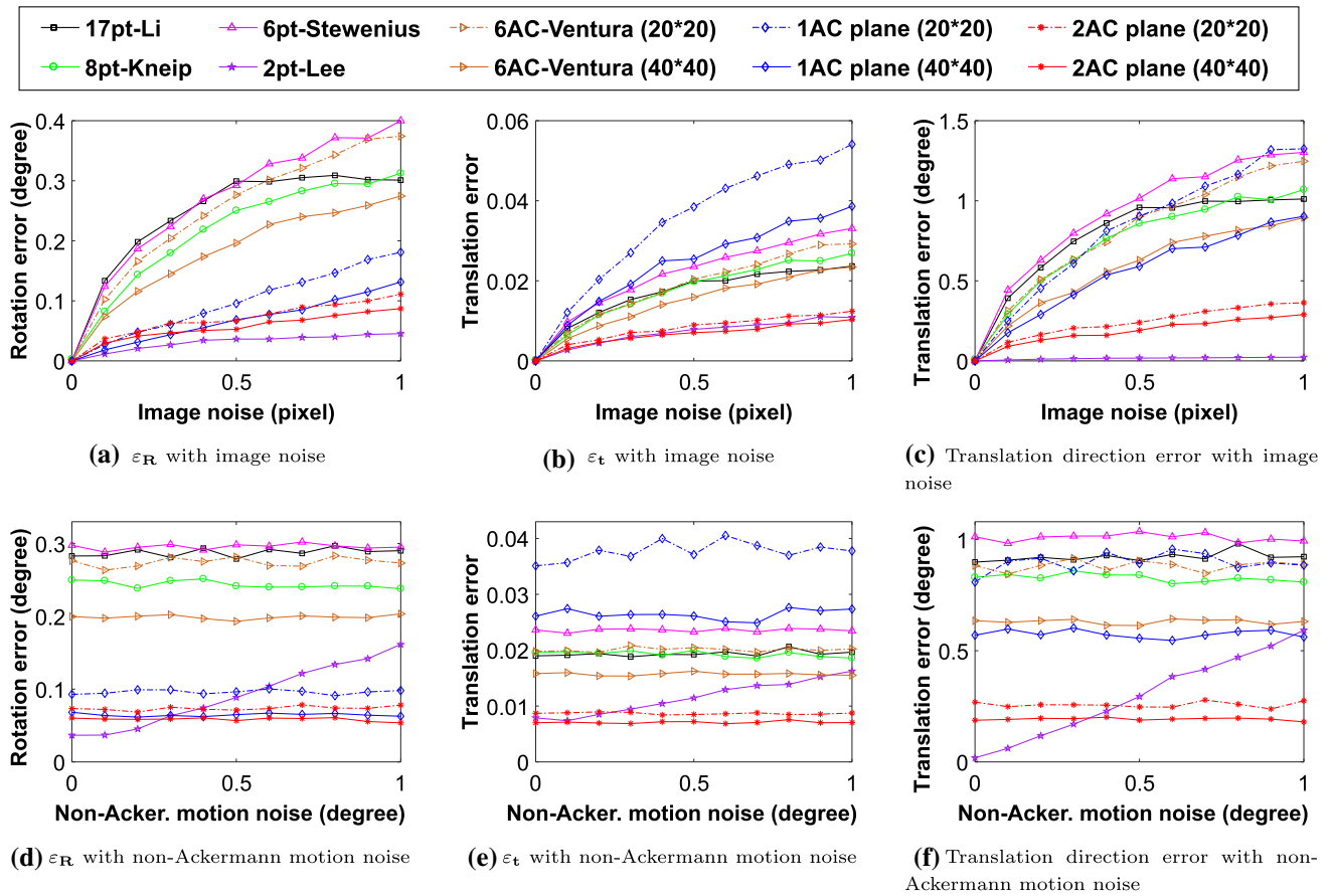
Fig. 12 Rotation and translation error under Ackermann motion. a–c Varying image noise under perfect Ackermann motion. d–f Varying non-Ackermann motion noise and fixed 0.5 pixel std. image noise
