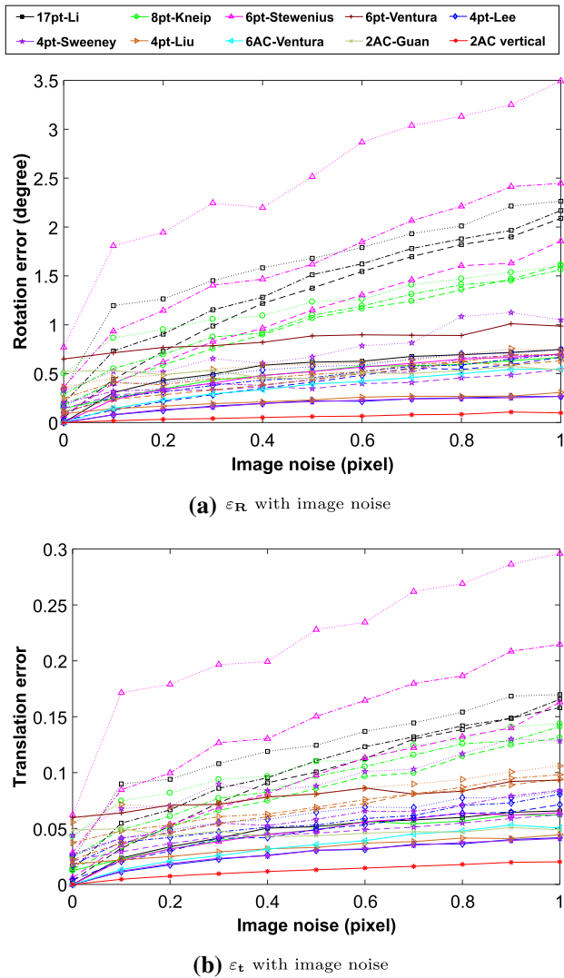
Fig. 14 Rotation and translation error with varying image noise under random motion with known vertical direction. Solid line indicates using image point pairs of ACs. Dashed line, dash-dotted line and dotted line indicate using the hallucinated PCs, which are generated with different distribution area w = 1, 5, 10 pixels, respectively
