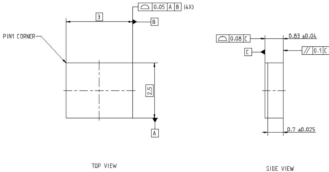
Figure 45 : Dimensions from top and side view
