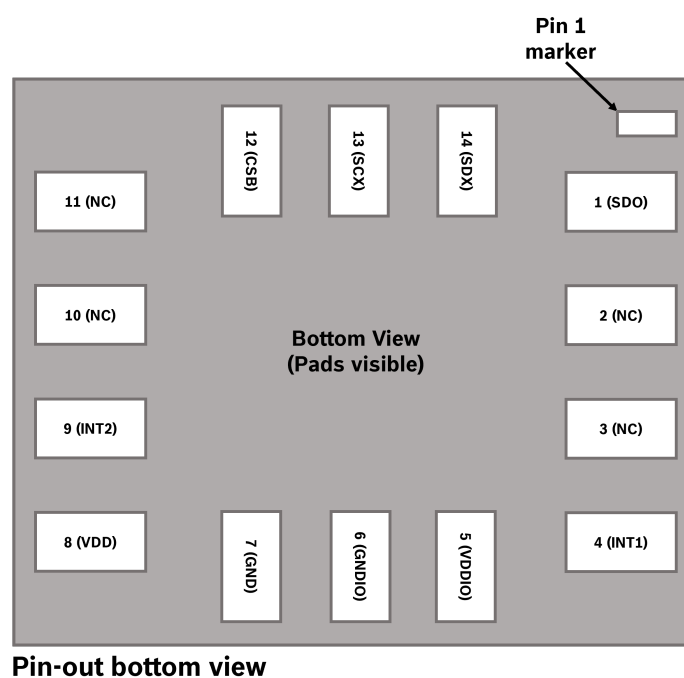
Figure 38 : Pin-out: bottom view
