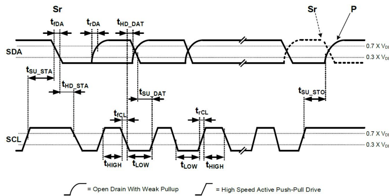
Figure 35 : I²C timing diagram
