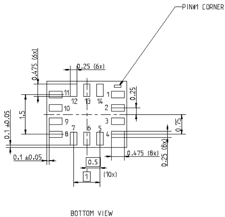
Figure 46 : Dimensions from bottom view
