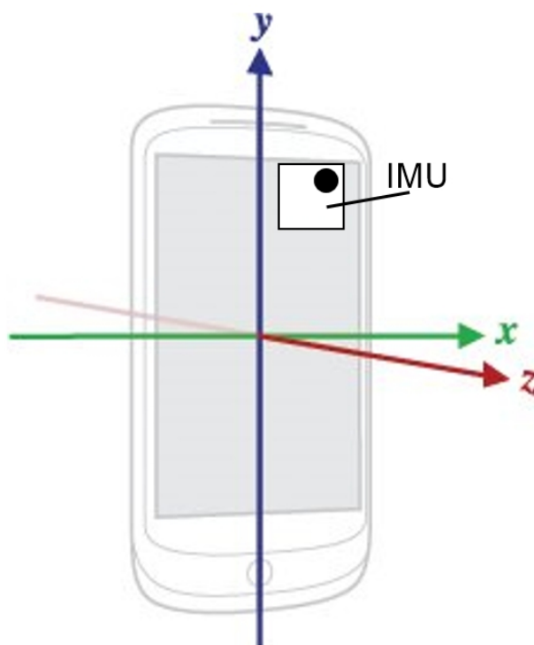
Figure 44 : Definition of the sensing axes orientation within a device
