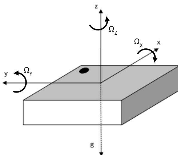
Figure 43 : Definition of the sensing axes orientation for the raw device
