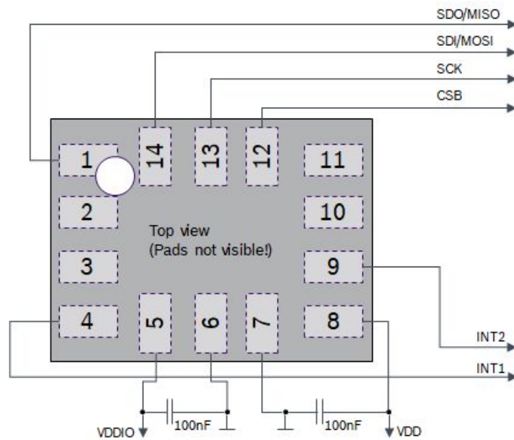
Figure 39 : 4-wire SPI connection
