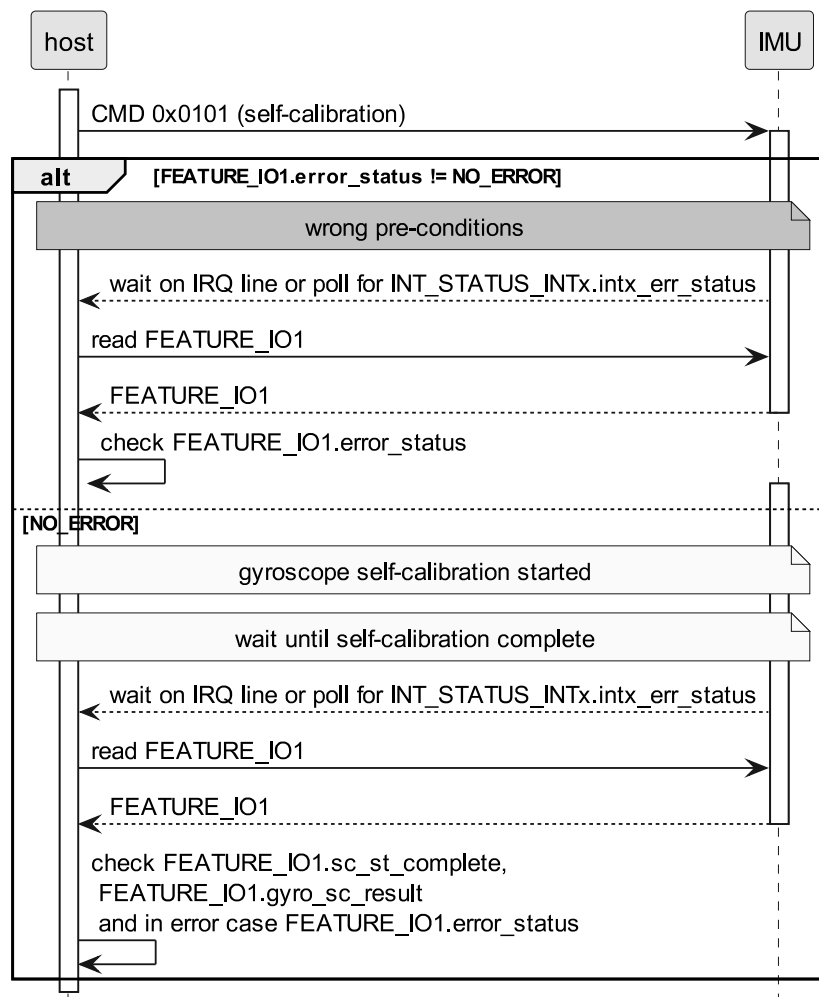
Figure 26 : Self-Calibration Start Sequence
