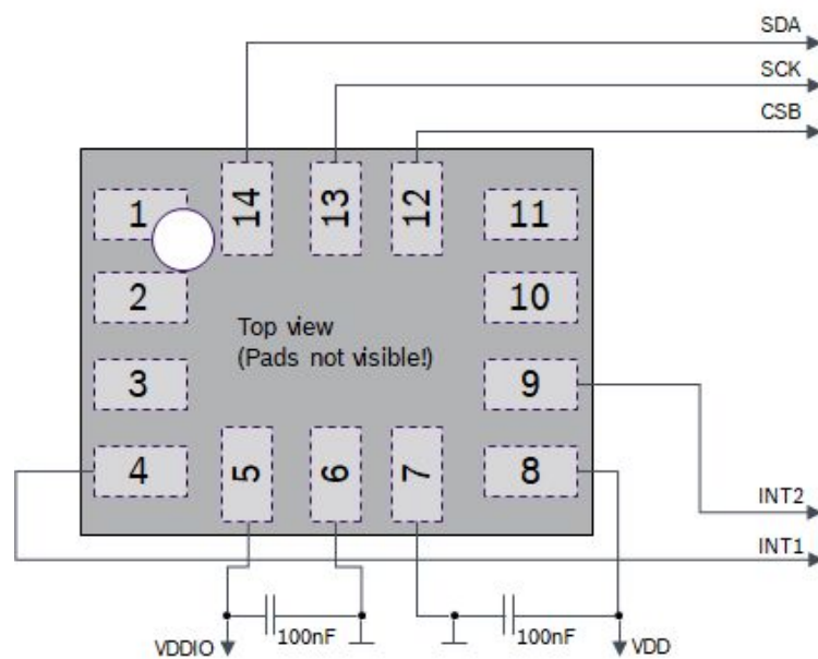
Figure 40 : 3-wire SPI connection
